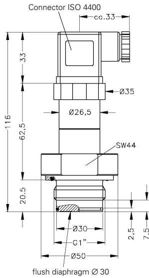
G1" flush with radial o-ring
